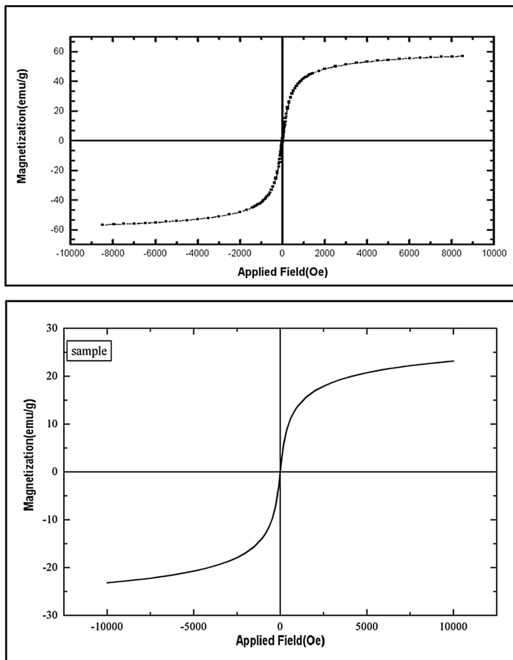
Fig. 4. The magnetic curves of \text{Fe}_3\text{O}_4 (upper) and \text{Cu-imine ligand@SiO}_2\text{@Fe}_3\text{O}_4 (lower).
