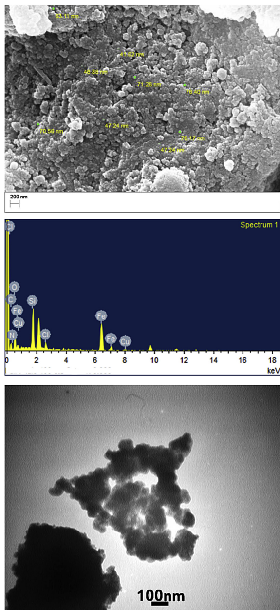
Fig. 1. SEM/EDAX elemental analysis and TEM image of Cu-imine ligand@ \text{SiO}_2@\text{Fe}_3\text{O}_4 .
