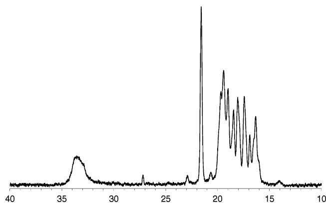
Figure 18. ^{31}\text{P} NMR spectra of \text{SiCl}_4 and 4b in \text{CD}_2\text{Cl}_2 at -70^\circ\text{C} .
