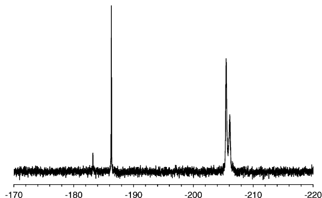
Figure 20. Portions of the 29 Si NMR spectra of SiCl 4 and 4a in CD 2 Cl 2 at -70^\circ\text{C} .
