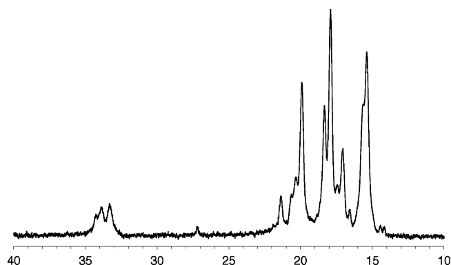
Figure 21. 31 P NMR spectra of SiCl 4 and 4a in CD 2 Cl 2 at -70^\circ\text{C} .
