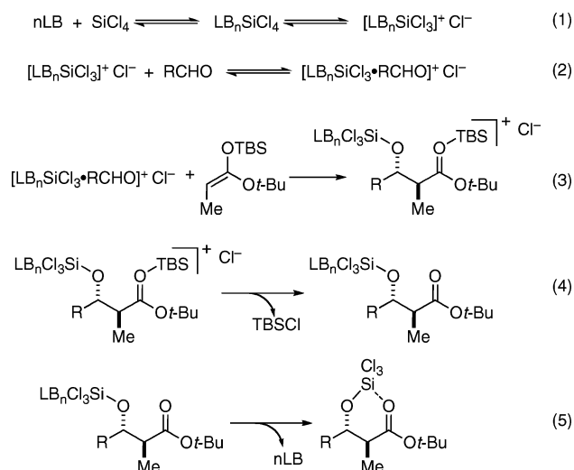
Figure 22. Generalized mechanism for the aldolization process.
