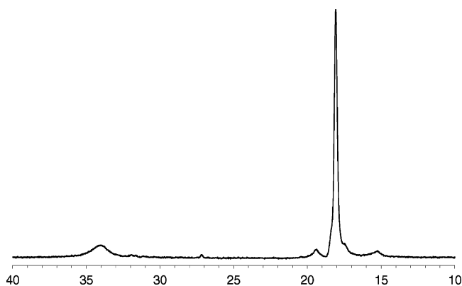
Figure 16. ^{31}\text{P} NMR spectra of \text{SiCl}_4 and 4d in \text{CD}_2\text{Cl}_2 at -70^\circ\text{C} .
