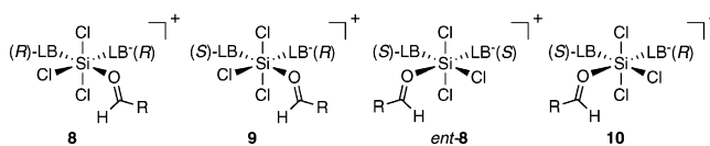
Figure 23. Reactive homo- and heterochiral mer -cis complexes of an aldehyde.
