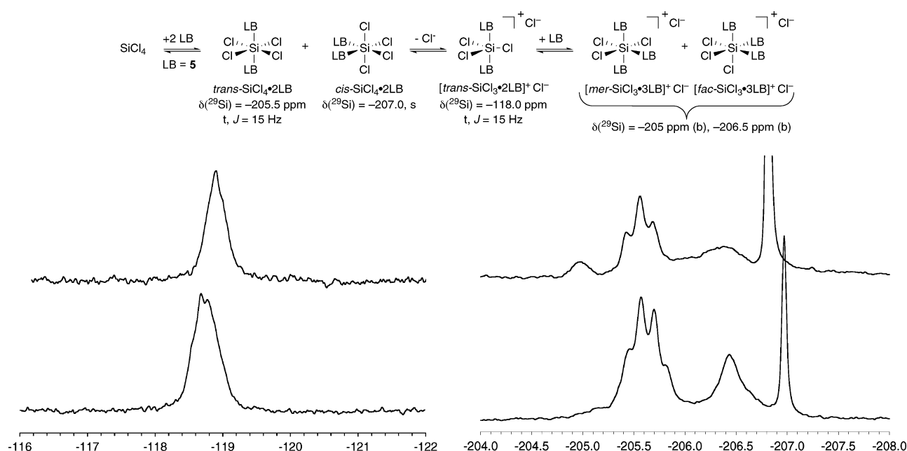
Figure 10. Portions of the ^{29}\text{Si} NMR spectra of \text{SiCl}_4 and 5 in \text{CD}_2\text{Cl}_2 at -70^\circ\text{C} . (Top) Enantiopure (R)- 5 . (Bottom) 54:46 mixture of (R)- and (S)- 5 , which gave an apparent diastereomer ratio of ca. 1:1.
