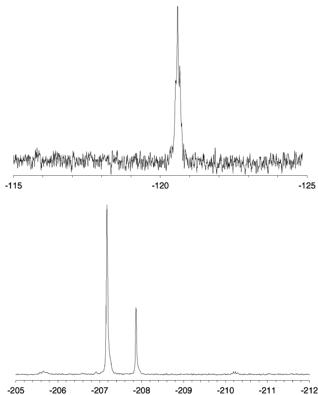
Figure 9. 29 Si NMR spectra of a mixture of SiCl 4 and HMPA in CD 2 Cl 2 at -70^\circ\text{C} .
