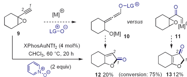
Scheme 1. First Attempt at Oxidative Cyclization with Alkynyl Oxirane Model Substrate 9 (LG = Nu in eq 2)
