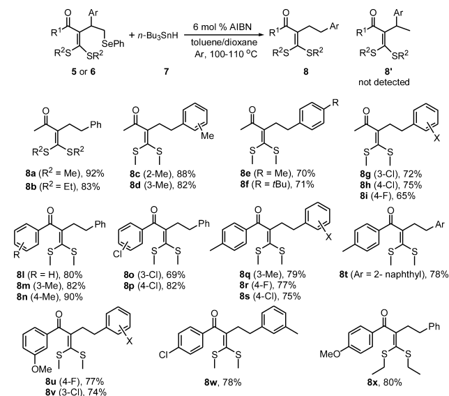
Scheme 5. Radical Dephenylselenative Aryl Transfer of 5 and 6 To Form Linear Hydrovinylation Products 8a–i
