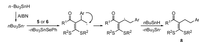
Scheme 6. Radical Reductive Aryl Transfer of 5 and 6
