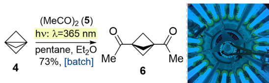
Scheme 3. Photochemical Synthesis of Diketone 6 in Batch a
