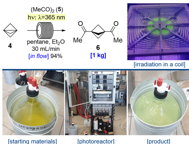
Scheme 4. Photochemical Synthesis of Diketone 6 in Flow a
