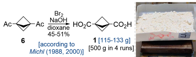
Scheme 5. Multigram Scale Synthesis of Diacid 1 in Batch
