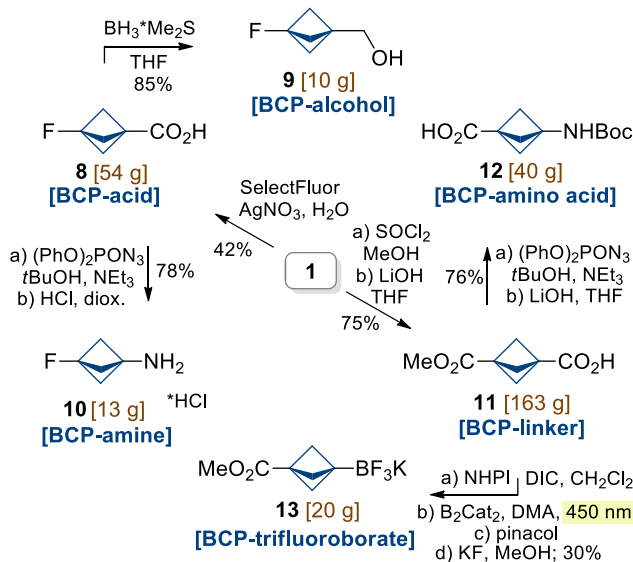
Scheme 6. Multigram Scale Synthesis of BCP-Containing Building Blocks 8 – 13 from Diacid 1
