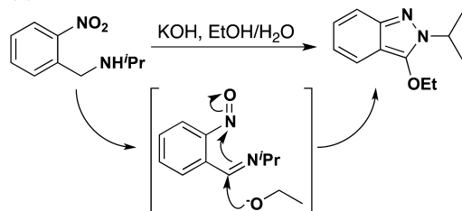
Figure 1. (a) Bioactive 2H-indazoles. (b) A typical Davis–Beirut reaction proceeding through the proposed nitrosoimine intermediate. 6
