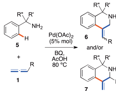
Scheme 5. Synthesis of Tetrahydroisoquinolines by Annulation of Benzylamines with Allenes
