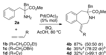
Scheme 4. Annulation of Allenes 1b–d with Amine 2a
