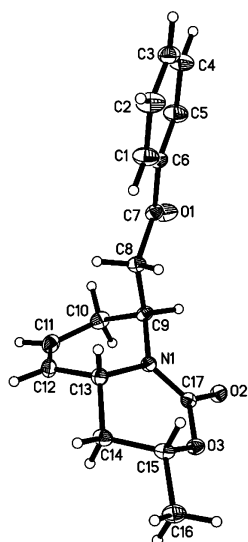
Figure 3. X-ray structure of piperidine 17a.
