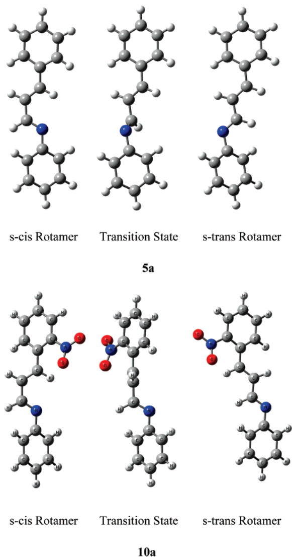
FIGURE 2. Optimized geometrical structures of s-trans, s-cis rotamers and the corresponding transition state between two forms of azidienes 5a and 10a calculated at the B3LYP/6-31G* level.
