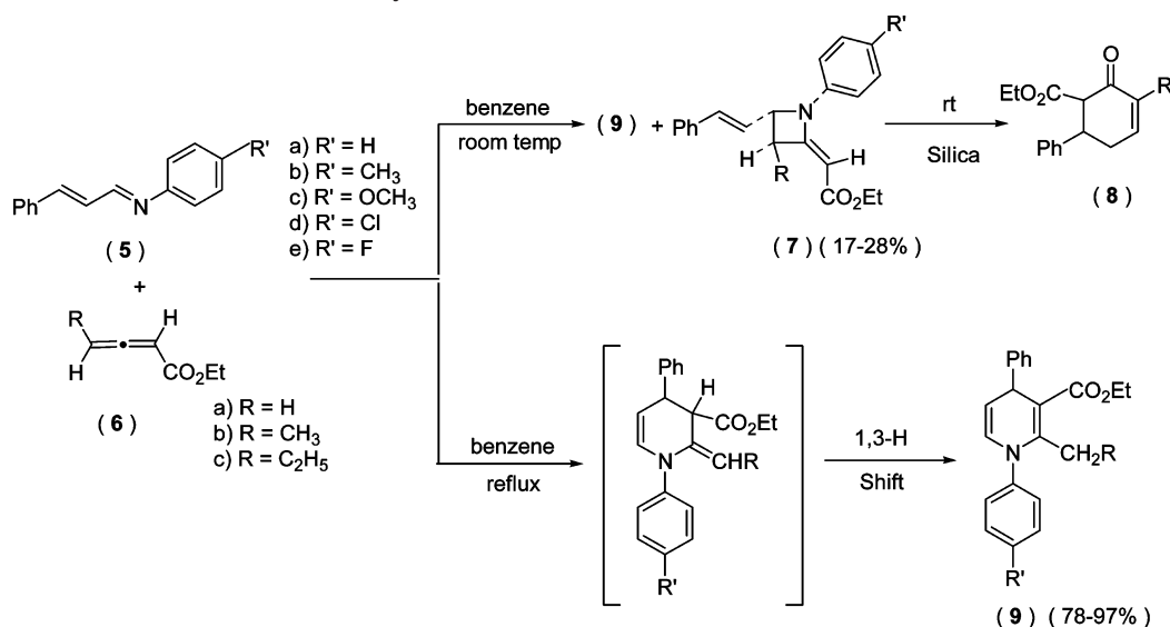
SCHEME 2. Thermal and Microwave Assisted Reactions of 1-Azadienes and Allenic Esters
