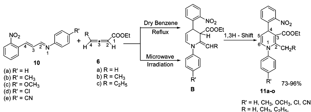
SCHEME 2. Thermal and Microwave Assisted Reactions of 1-Azadienes and Allenic Esters
