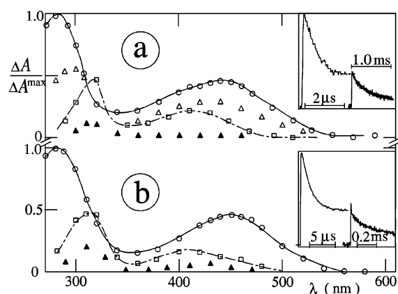
Figure 4. Transient absorption spectra of 2,6-Me 2 BQ (1 mM) in argon-saturated (a) aqueous solution at pH 7, (b) HFP-water (1:1) at 20 ns (○), 1 \mu s (Δ), 10 \mu s (□), and 1 ms (▲) after the 308-nm pulse; insets: triplet and radical decay at 430 nm.
