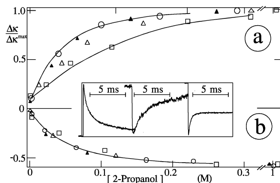
Figure 10. Dependences of the conductivity signal at 0.1 ms on [2-propanol] for BQ (circles), MeBQ (squares), and 2,6-Me 2 BQ (triangles) in argon-saturated aqueous solution (open) and mixed with acetonitrile (1%, full) at (a) pH 5 and (b) pH 9, \lambda_{\text{exc}} = 248 nm; insets: conductivity signals for BQ at pH 5, 8, and 9.5 (from left to right).
