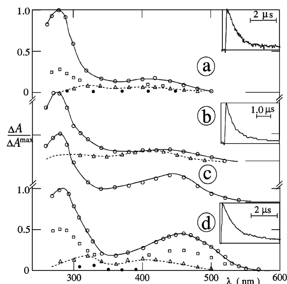
Figure 7. Transient absorption spectra of (a) BQ, (b) MeBQ, (c) 2,5-Me 2 BQ, and (d) 2,6-Me 2 BQ in argon-saturated aqueous solution at pH 6–7 at 20 ns (○), 1 μs (□), 10 μs (Δ), and 0.1 ms (●) after the 248-nm pulse; insets: triplet decay at 290 nm.
