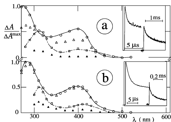
Figure 3. Transient absorption spectra of BQ (1 mM) in argon-saturated (a) aqueous solution at pH 7, (b) HFP-water (1:1) at 20 ns (○), 1 \mu s (Δ), 10 \mu s (□), and 1 ms (▲) after the 308-nm pulse; insets: triplet and radical decay at 420 nm.
