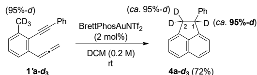
Scheme 5. Isotopic labeling experiment
