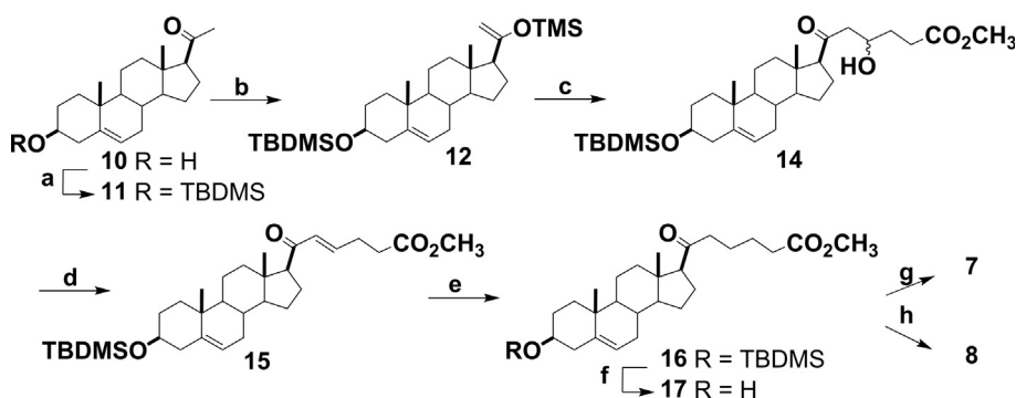
Scheme 1. Reagents and conditions: a) TBDMSCl, imidazol, DMF, 92.0%; b) i) LDA-THF, ii) TMSCl, -78^\circ\text{C} to room temperature; c) \text{HCOCH}_2\text{CH}_2\text{COOCH}_3 ( 13 ), 61.0% from 11 ; d) i) \text{MsCl} , Py, 98.0%, ii) DBU, acetone, 81.0%; e) \text{H}_2 , Pd 10% \text{C} , EtOAc, 1 Bar, room temperature, 96.0%; f) HF 40%, \text{CH}_3\text{CN} , 90.0%; g) i) PCC, \text{CH}_2\text{Cl}_2 , 80.0%; ii) HCl 1 N, THF, 55.0%; h) LiOH, \text{H}_2\text{O-THF-MeOH} , 92.0%.
