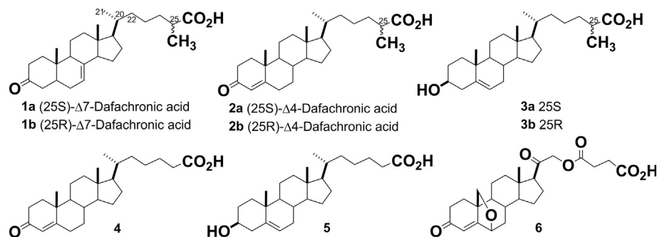
Fig. 1. Structures of compounds 1–6.
