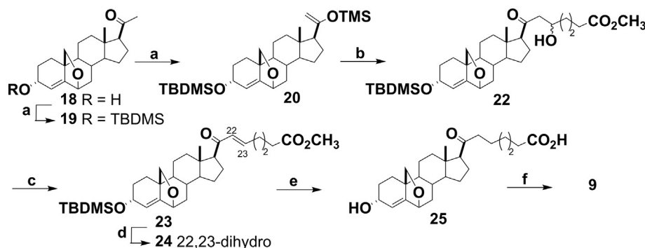
Scheme 2. Reagents and conditions: a) i) TBDMSCl, imidazol, DMF, 92.0%, ii) 1) LDA-THF, 2) TMSCl, -78^{\circ}\text{C} to room temperature; b) \text{HCO}(\text{CH}_2)_3\text{COOCH}_3 ( 21 ), 64% from 19 ; c) i) triflic anhydride, \text{CH}_2\text{Cl}_2 -Py, ii) DBU, acetone, 47.0%; d) \text{H}_2 , Pd 10% C, EtOAc, 1 Bar, room temperature, 77.0%; e) i) ClH 6 N, THF, ii) NaOH 50% (aq), 65%; f) \text{MnO}_2 , \text{CH}_2\text{Cl}_2 , 62%.
