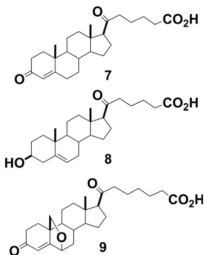
Fig. 2. Structures of compounds 7 and 8, 20-keto analogues of bioactive steroids 4 and 5 respectively and compound 9, a non-hydrolysable analogue of 6.
