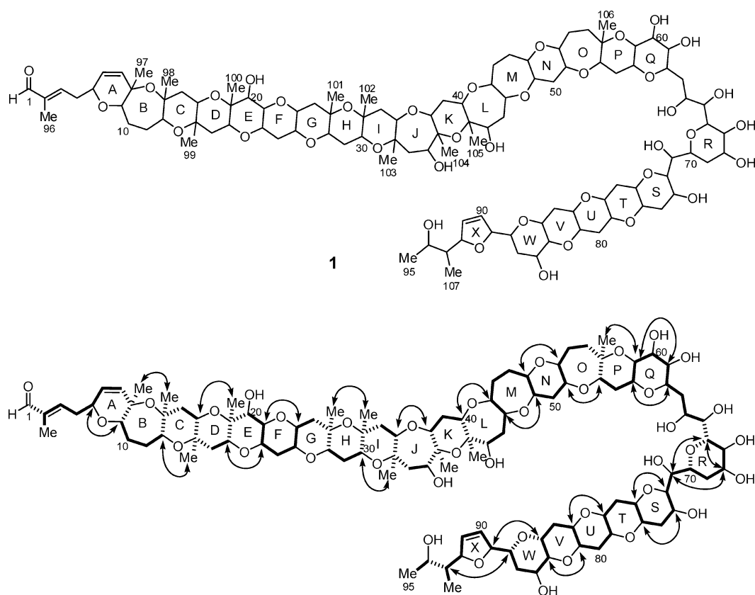
Figure 1. Structure and NMR interpretation of brevisulcenal-F ( 1 ). Bold lines indicated connectivities elucidated on the basis of the ^1\text{H} – ^1\text{H} COSY and TOCSY data. Double-headed arrows show the important NOE correlations observed in the NOESY spectra of 1 . Broken lines depicted the key HMBC correlations of 1 .
