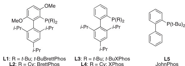
Figure 1. Biarylphosphine ligands.
