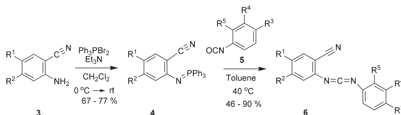
Scheme 1. General Method for the Synthesis of Heteroenyne-allenes 6
