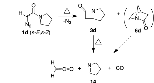
Scheme 12. Thermal Formation and Decomposition of \beta -Lactam 3d and Possibly 6d
