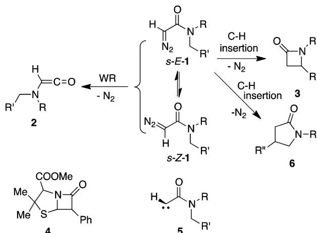
Scheme 1. Wolff Rearrangement (WR) and C–H Insertion Reactions of Diazoamides
