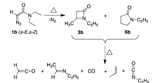
Scheme 11. Formation and Thermal Decomposition of Lactams 3b and 6b
