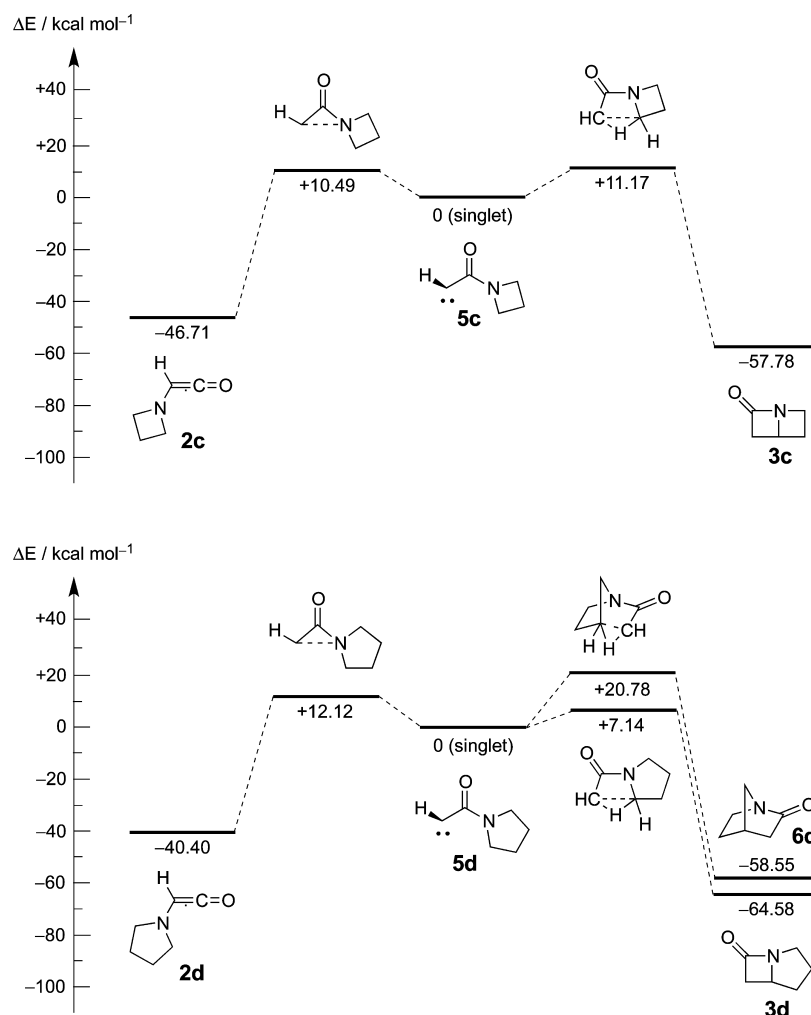
Figure 13. Relative calculated energies ( \text{kcal mol}^{-1} , B3LYP/6-31G(d)) of products and transition states arising from diazoamides 1c,d . For each series the respective singlet carbene 5 is set to 0 \text{ kcal mol}^{-1} . Note: the carbene C–H bond is perpendicular to the planar amide moiety (see the Supporting Information for computational details).
