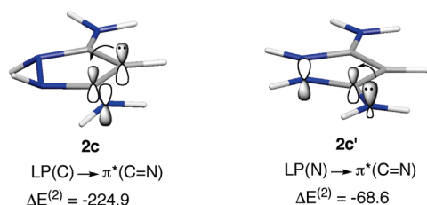
Figure 6. Two-electron interactions and associated second-order perturbation energies, \Delta E^{(2)} (in kcal/mol) for 2c and 2c' cations.
