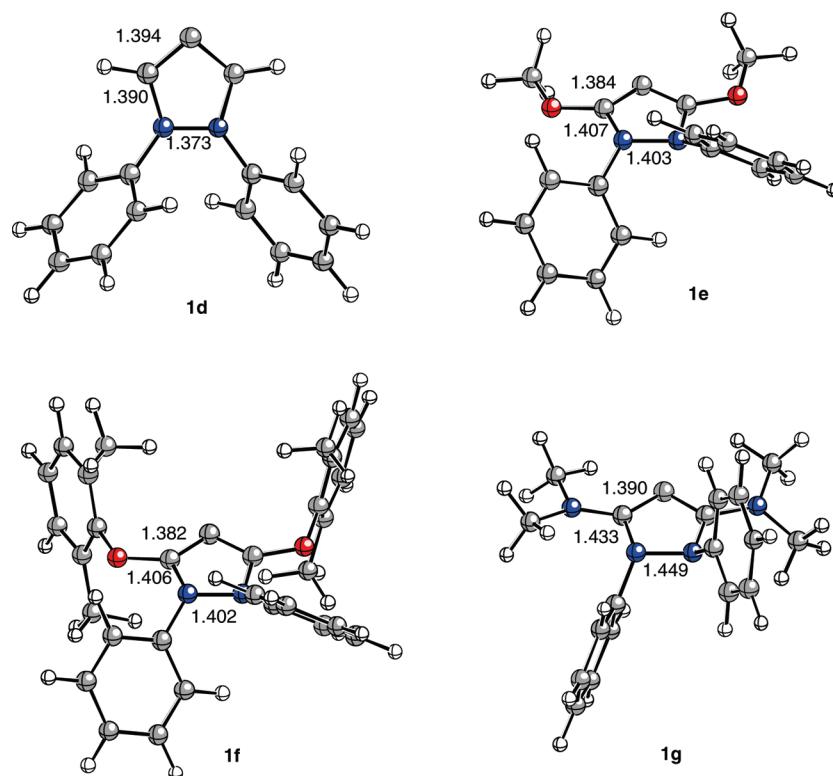
Figure 2. Ball and stick representations of the bent allenenes 1d–g . All structures correspond to fully optimized RI-BP/def2-TZVPP geometries. Bond distances are given in Å. White, gray, red, and blue colors denote hydrogen, carbon, oxygen, and nitrogen atoms, respectively.
