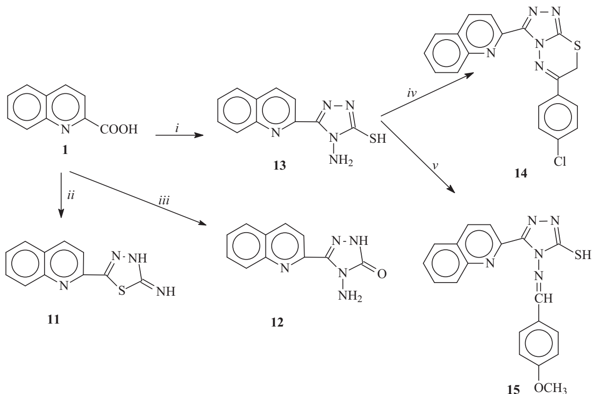
Scheme 2. Synthesis of compounds 11-15 . i ) thiocarbonylhydrazide, ii ) thiosemicarbazide, iii ) carbonylhydrazide, iv ) 4-chlorophenacylbromide, v ) 4-methoxybenzaldehyde.
