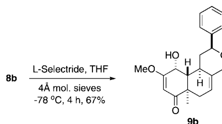
SCHEME 5. Attempted Conjugate Reduction of Epimerized Adduct 8b
