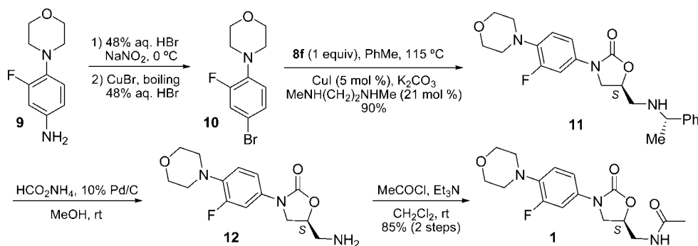
Scheme 3. Synthesis of Enantiopure Linezolid, 1 , from the 1,3-Oxazolidin-2-one (3'S,5S)- 8f
