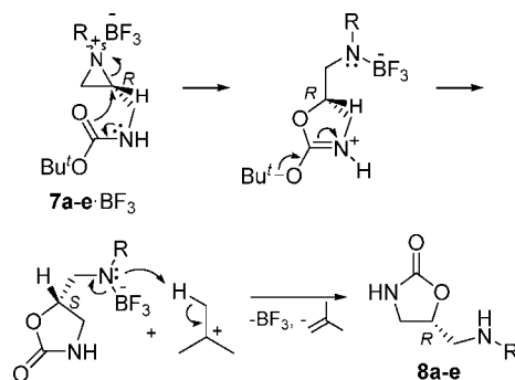
Scheme 2. Probable Mechanism for the Intramolecular Ring-Opening Step
