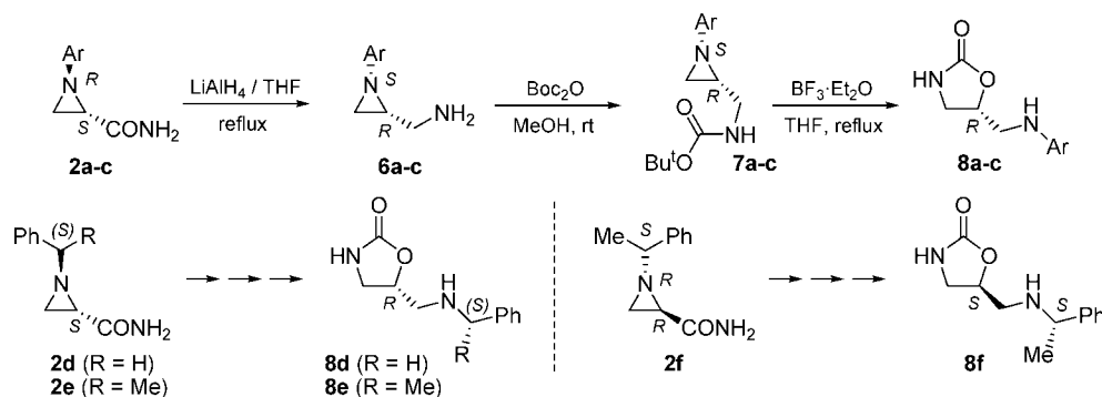
Scheme 1. Three-Step Preparation of Enantiopure 1,3-Oxazolidin-2-ones 8 from Enantiopure Aziridine-2-carboxamides 2
