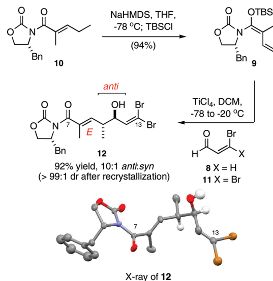
Scheme 2. Synthesis of the C7–C13 Region via an Asymmetric Vinylogous Mukaiyama Aldol Reaction
