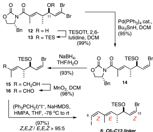
Scheme 3. Synthesis of C6–C13 Cross-Coupling Linker
