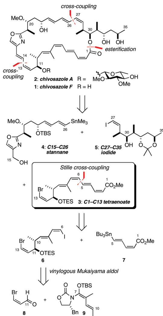
Scheme 1. Retrosynthetic Analysis
