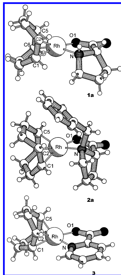
Figure 1. X-ray structures of 1a , 2a , and 3 .
