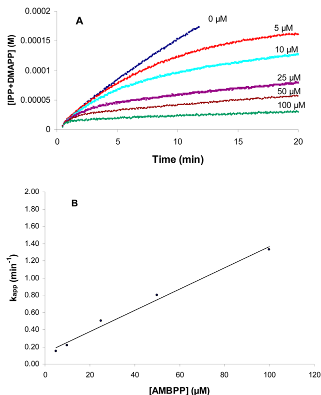
Figure 3. (A) Progress curves for inhibition of IspH by AMBPP. The reaction mixture contained NADPH (2 mM), IspH (0.5 \mu M), HMBPP (200 \mu M), FpR1 (17 \mu M), FldA (41 \mu M) in 50 mM Tris HCl buffer, pH 8, and varying concentrations of AMBPP from 0 to 100 \mu M. After preincubation for 3 min at 37 ^{\circ} C, IspH was added with a gastight syringe to initiate the reaction. Samples were prepared in a glovebox. (B) A plot of k_{app} versus [AMBPP] obtained by fitting the progress curves to eq 1.
