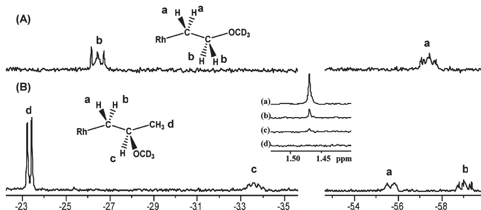
Figure 6. High-field 1 H NMR resonances for (A) (TSPP)Rh-CH 2 -CH 2 -OCD 3 and (B) [(TSPP)Rh-CH 2 -CH(OCD 3 )-CH 3 ]. (Inset: Observation of the β-OCH 3 group in (TSPP)Rh-CH(CO 2 CH 3 )-CH 2 -OCH 3 and very slow exchange of the -OCD 3 group in CD 3 OD. (a) t = 0 , (b) t = 1 month, (c) t = 2 months, and (d) t = 3 months.)
