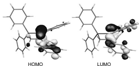
Figure 2. Contour plots of the frontier orbitals of 6a at 0.05 cut-off level (Molekel). [18]
