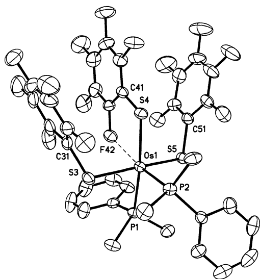
Fig. 1. Structure of [Os(SC 6 F 4 (F-2))(SC 6 F 5 ) 2 (PMe 2 Ph) 2 ] ( 1a ). (Ellipsoids at 30% probability levels. Hydrogen atoms were omitted for clarity.)
