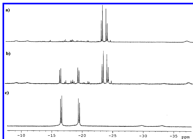
Figure 3. ^{31}\text{P}\{^1\text{H}\} NMR spectra (central part) of cis -[(PMe 2 Ph) 2 Pt(μ-OH) 2 (NO 3 ) 2 ] and 1-MeCy (1:2 molar ratio) in DMSO- d_6 at 27 °C: (a) fresh solution; (b) after 45 h; (c) after 3 weeks at room temperature.
