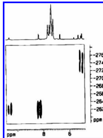
Figure 8. ^{15}N – ^1H HMBC spectra (low field) of 4 in DMSO-d_6 .
