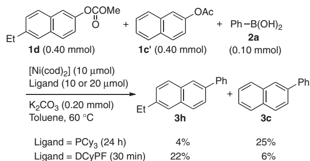
Scheme 1. Competitive experiment of the cross-coupling reaction.
