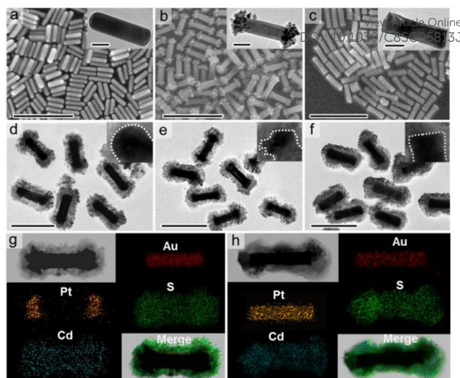
Fig. 1 SEM images of (a) Au NRs, (b) Au-Pt, and (c) Au@Pt, scale bar, 200 nm. The insets of (a-c) show TEM images of corresponding samples, scale bar, 20 nm. TEM images of (d) Au@CdS, (e) Au-Pt@CdS and (f) Au@Pt@CdS, scale bar, 200 nm. Elemental mapping results of (g) Au-Pt@CdS and (h) Au@Pt@CdS.
