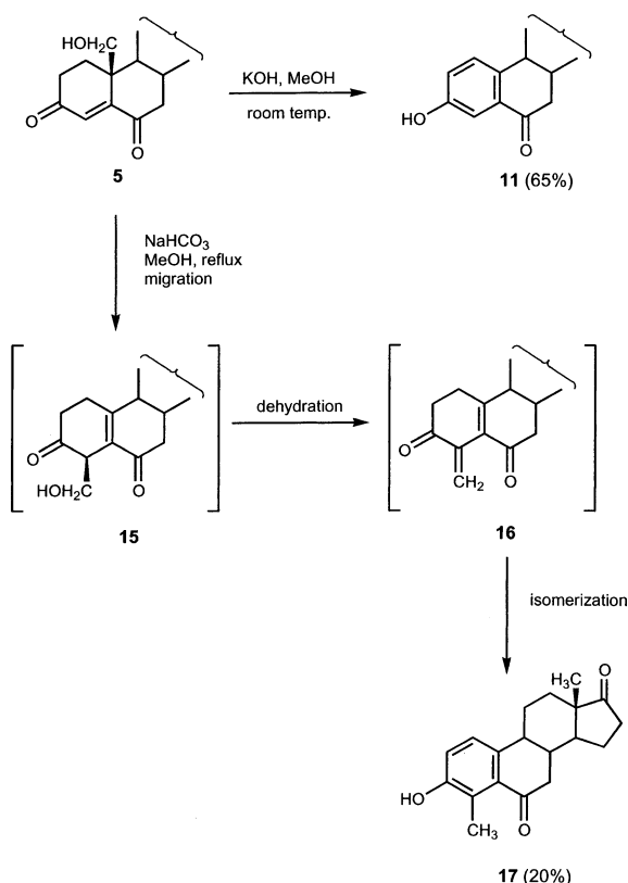
Fig. 2. Reaction of 19-Hydroxy Steroid 5 with a Base
