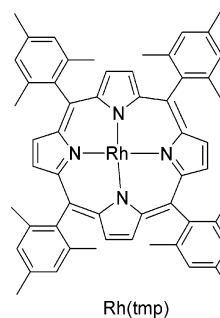
Figure 1. Structure of Rh(tmp).
