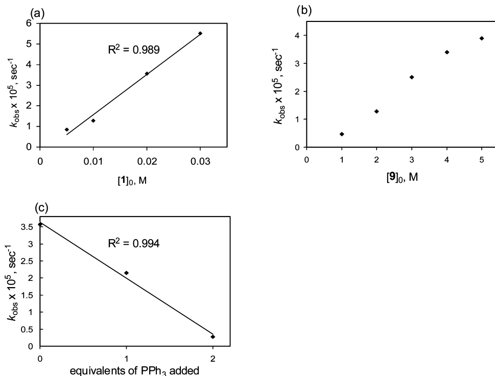
Figure 7. Dependence of the initial concentration of the ruthenium complex ( [1]_0 ), the initial concentration of trimethylvinylsilane 9 ( [9]_0 ), and the concentration of \text{PPh}_3 added ( [\text{PPh}_3] ) as a rate constant k_{\text{obs}} in the alkylation of 10 with 9 at 25 °C. (a) Plotting k_{\text{obs}} versus [1]_0 . Reaction conditions: [10]_0 = 0.10 \text{ M} , [1]_0 = 5.0\text{--}30 \text{ mM} , [9]_0 = 2.0 \text{ M} , benzene- d_6 . (b) Plotting k_{\text{obs}} versus [9]_0 . Reaction conditions: [10]_0 = 0.10 \text{ M} , [1]_0 = 0.01 \text{ M} , [9]_0 = 1.0\text{--}5.0 \text{ M} , benzene- d_6 . (c) Plotting k_{\text{obs}} versus equivalents of \text{PPh}_3 added. Reaction conditions: [10]_0 = 0.10 \text{ M} , [\text{Ru}]_0 = 0.02 \text{ M} , [9]_0 = 2.0 \text{ M} , \text{PPh}_3 = 0\text{--}2 equiv to the ruthenium complex, benzene- d_6 .
