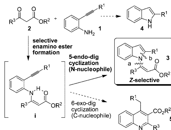
SCHEME 2. Strategy
