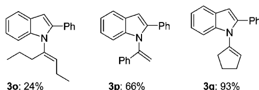
FIGURE 1. Products from simple ketones.
