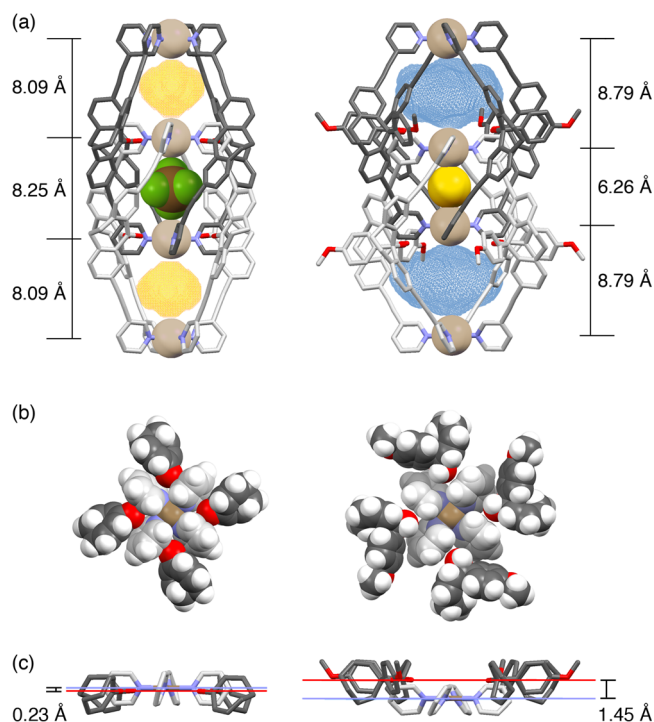
Figure 3. (a) Comparison of the X-ray structures of [BF 4 @Pd 4 L 1 8 ](BF 4 ) 7 (left) 12 and [Cl@Pd 4 L 2b 8 ](BF 4 ) 7 (right). Color scheme: C, light/dark gray; N, blue; O, red; Cl, yellow; F, green; B, brown; Pd, beige. For clarity, H atoms, solvent molecules, and anions not in the central pockets have been omitted. (b) Space-filling top views and (c) stick side views of the inner Pd(py) 4 planes (H atoms omitted) illustrating the differences in the relative positions of the interpenetrating cage fragments in [BF 4 @Pd 4 L 1 8 ](BF 4 ) 7 (left) and [Cl@Pd 4 L 2b 8 ](BF 4 ) 7 (right). In (c), the distances between the N 4 and O 4 planes are given.
