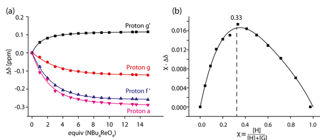
Figure 4. (a) Plot of 1 H NMR signal shifts observed in the titration of [Cl@Pd 4 L 2a 8 ](BF 4 ) 7 with NBu 4 ReO 4 (CD 3 CN, 293 K). (b) Job plot analysis showing a ReO 4 - :[Cl@Pd 4 L 2a 8 ] ratio of 2:1.
