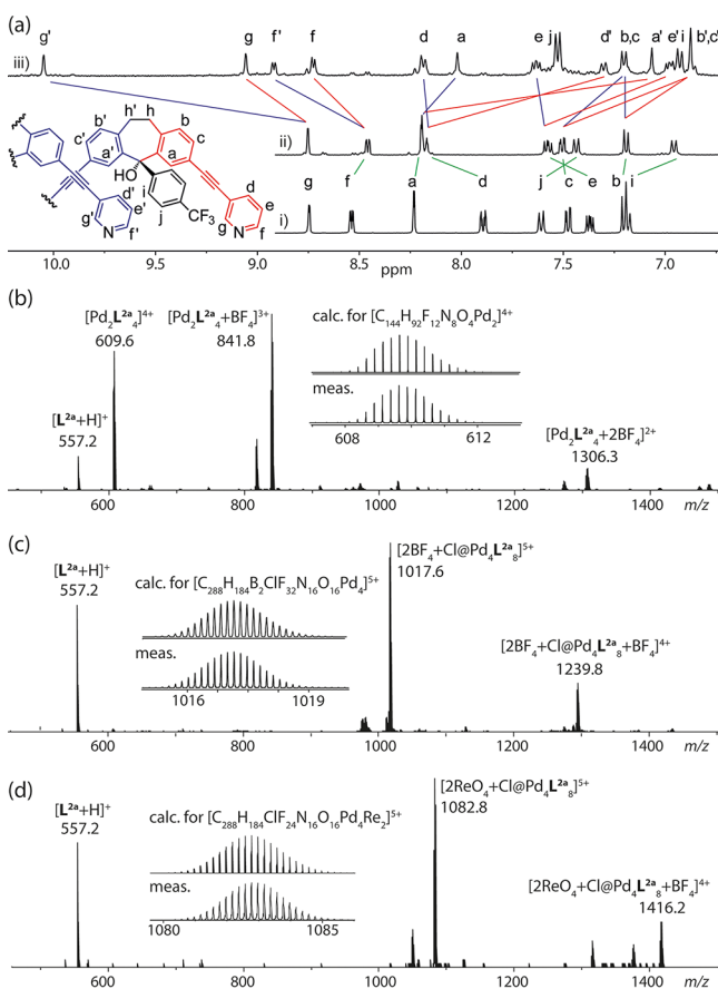
Figure 2. (a) 1 H NMR spectra of (i) ligand L 2a , (ii) monomeric cage [Pd 2 L 2a 4 ](BF 4 ) 4 , and (iii) dimeric cage [Cl@Pd 4 L 2a 8 ](BF 4 ) 7 (400 MHz, 298 K, CD 3 CN). (b–d) ESI-FTICR mass spectra of (b) monomeric cage [Pd 2 L 2a 4 ](BF 4 ) 4 , (c) double cage [2BF 4 +Cl@Pd 4 L 2a 8 ](BF 4 ) 5 , and (d) the host–guest complex [2ReO 4 +Cl@Pd 4 L 2a 8 ](BF 4 ) 5 .
