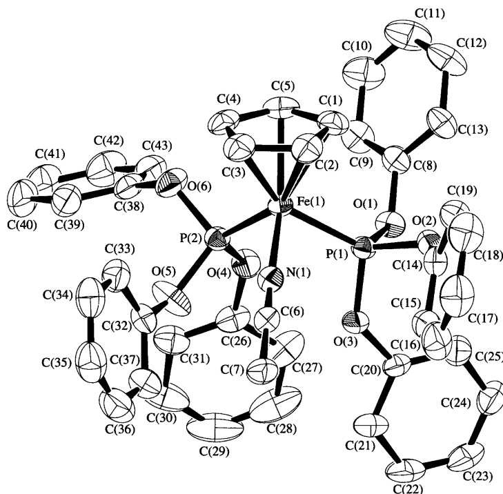
Fig. 1. Molecular structure of complex 9a . Hydrogen atoms and \text{PF}_6^- have been omitted for clarity.
