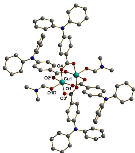
Figure 1. Molecular structure of 5 with hydrogen atoms omitted for clarity.
