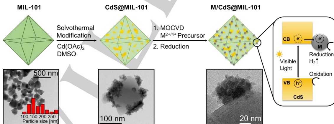
Scheme 2. Synthesis of the photocatalyst M/CdS@MIL-101. The decoration with CdS semiconductor particles proceeds via a solvothermal modification. The metal precursor (Ni: Ni(C 5 H 5 ) 2 ; Pd: Pd(C 3 H 5 )(C 5 H 5 ); Pt: Me 3 Pt(CH 3 -C 5 H 4 )) is infiltrated into MIL-101 (green) by gas phase deposition and reduced by hydrogen treatment. In the semiconductor CdS (yellow) an electron is promoted from the valence band (VB) to the conduction band (CB) by the absorption of visible light. After the directed electron transfer toward the metal particles (grey), spatially separated redox reactions can be catalysed.
