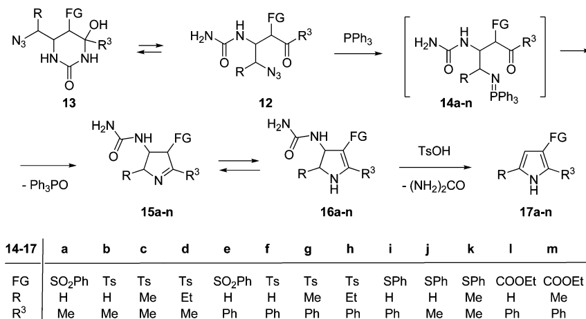
Scheme 3. Synthesis of Pyrrolines and Pyrroles via Staudinger/aza-Wittig Reaction
