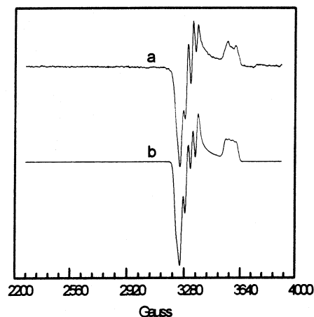
Fig. 1. EPR spectrum of the species deriving from the reaction of \text{Ir}(\text{Me})_2\text{Cp}^*(\text{PMe}_3) ( 1d ) with \text{NOBF}_4 in \text{CH}_2\text{Cl}_2 . (a) Observed spectrum; (b) simulated spectrum.
