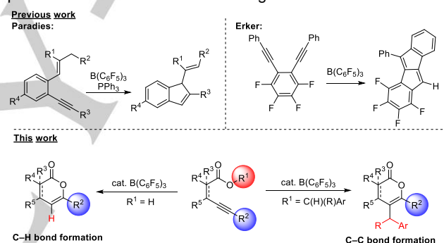
Scheme 1. Examples of B(C 6 F 5 ) 3 catalysis.
