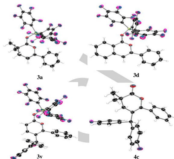
Figure 2. Solid-state structure of compound 3a , 3d , 3v and 4c . Disordered F atom modelled over two sites ( 3v and 4c ). Thermal ellipsoids shown at 50% probability.
