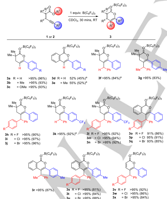
Scheme 2. Substrate scope for the cyclization reaction of 1 with B(C_6F_5)_3 .
