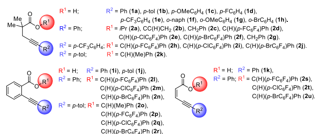
Figure 1. Substrates 1 and 2 used in this study.
