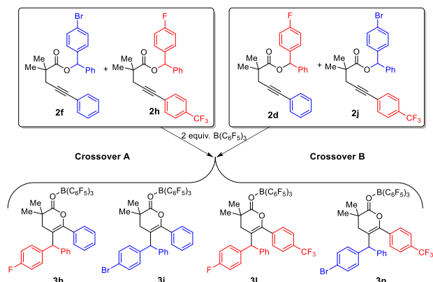
Scheme 5. Crossover reactions.
