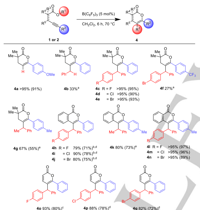
Scheme 4. Tandem catalytic one-pot cyclization/hydrosilylation to yield 6 .
