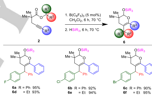
Scheme 4. Tandem catalytic one-pot cyclization/hydrosilylation to yield 6 .
