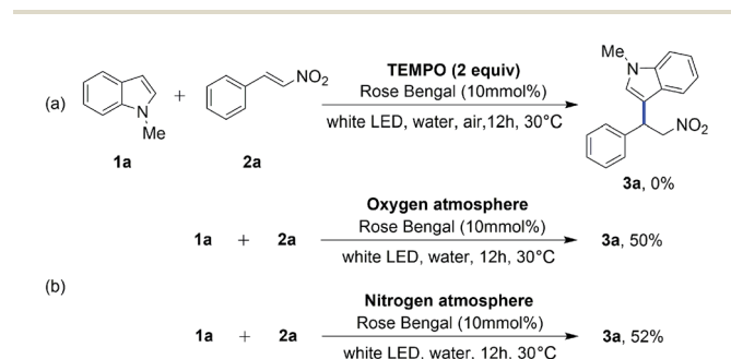
Scheme 3 Control experiment.
