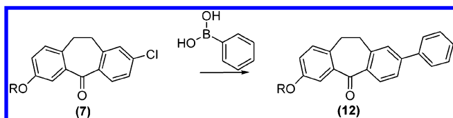
Scheme 2. Suzuki Coupling a
