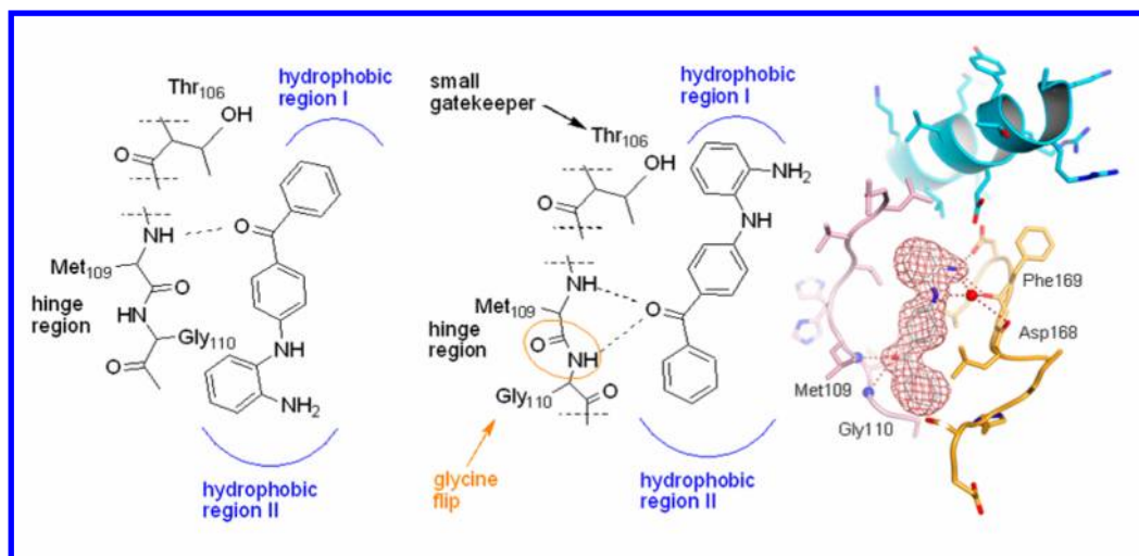
Figure 3. Binding mode of 2-amino-phenyl-amino-benzophenone. Left: Schematic binding mode according to Ottosen et al. 21 Middle: Schematic binding mode suggested by our group. Right: Crystal structure of 2-amino-phenyl-amino-benzophenone in complex with p38 \alpha MAP kinase (PDB ID 3QUD), confirming the binding mode suggested by our group.
