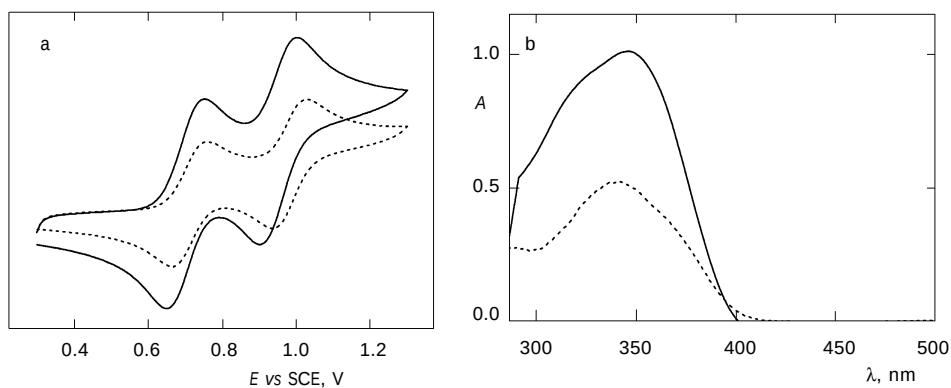
FIG. 3 Cyclic voltammograms (a) and UV-VIS spectra (b) of 2 (dashed lines) and 5 (full lines) measured in \text{CH}_2\text{Cl}_2/0.1 \text{ M TBAPF}_6 at the same concentrations ( 0.001 \text{ mol l}^{-1} )
