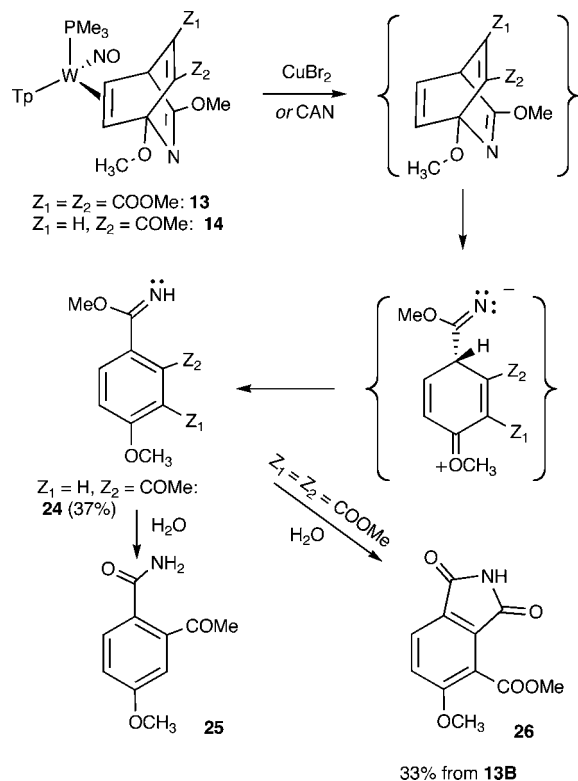
Scheme 4. Oxidative Decomplexation of Azabarrelene Complexes (13 and 14)
