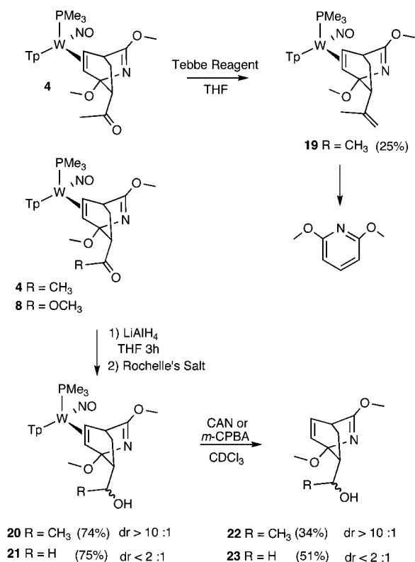
Scheme 3. Reduction and Decomplexation of 4 and 8
