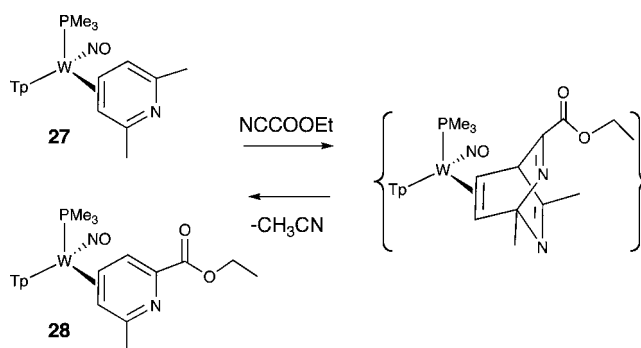
Scheme 6. Examples of Pyridine and Azoniaanthracene Cycloaddition
