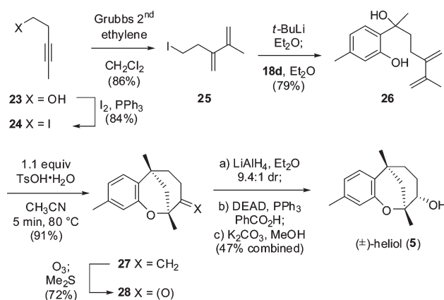
Figure 5. Total synthesis of (±)-heliol ( 5 ).
