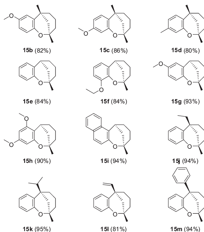
Figure 3. Analogues made from respective starting materials 12b–m . Isolated yields given in parentheses.
