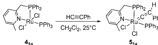
Scheme 4. Representative Reaction of Type 4 1x Phosphinopyridine Ru(II) Complexes with a Terminal Alkyne; Stoichiometric Reaction of RuCl 2 (L 1a )(PPh 3 ) ( 4 1a ) (mixture of cis and trans derivatives) with Phenylacetylene Giving the Corresponding Vinylidene Species RuCl 2 (L 1a )(CCHPh)(PPh 3 ) ( 5 1a ) Obtained as a Unique Single Isomer
