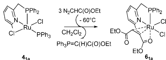
Scheme 5. Reaction of \text{RuCl}_2(\text{L}^{1a})(\text{PPh}_3) ( \mathbf{4}_{1a} ) (mixture of cis and trans isomers) with an Excess of Ethyl Diazoacetate Giving the Diethyl Maleate Complex \text{RuCl}_2(\text{L}^{1a})\{\text{cis-EtO}(\text{O})\text{C}(\text{H})\text{C}=\text{C}(\text{H})\text{C}(\text{O})\text{OEt}\} ( \mathbf{6}_{1a} ) as a Unique Isomer
