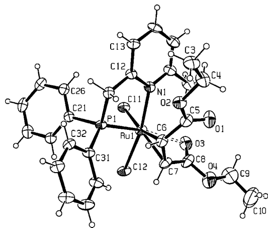
Figure 6. Perspective view of complex \text{RuCl}_2(\text{L}^{1a})\{\text{cis-EtO}(\text{O})\text{C}(\text{H})\text{C}=\text{C}(\text{H})\text{C}(\text{O})\text{OEt}\} ( \mathbf{6}_{1a} ). Ellipsoids are shown at the 30% probability level.
