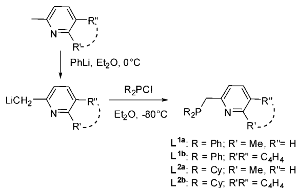
Scheme 1. General Synthetic Procedure and Labeling Scheme for Various 2-(Phosphinomethyl)pyridine Type Ligands
