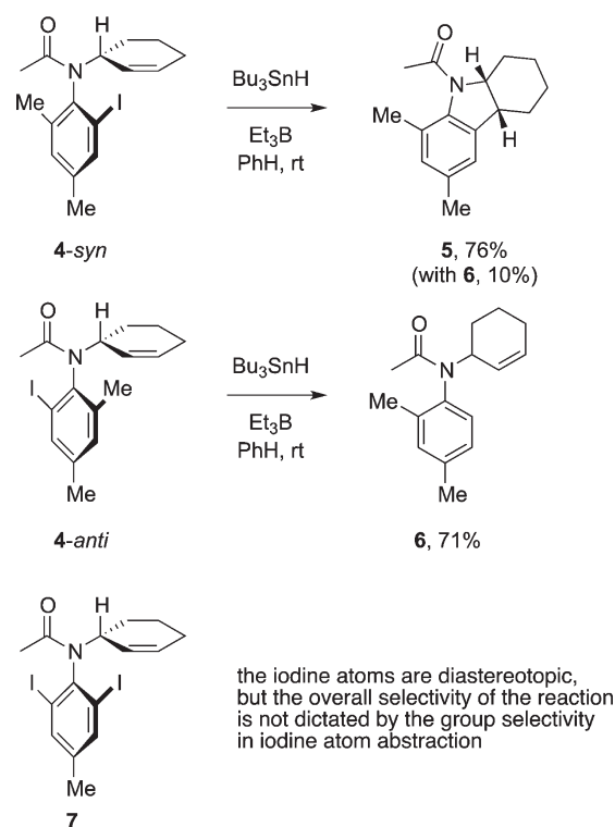
Figure 3. Precursor 7 designed on the basis of widely differing outcomes in radical reactions of atropisomers 4-syn and 4-anti .
