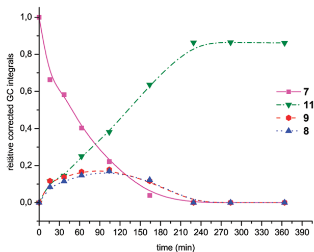
Figure 5. Concentration profiles of major products in the \text{Bu}_3\text{SnH} -mediated reaction of diiodoanilide 7 .
