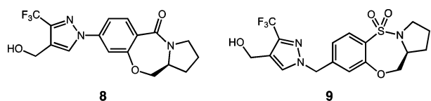
Chart 3. Additional Hybrid Compounds Targeted for Synthesis
