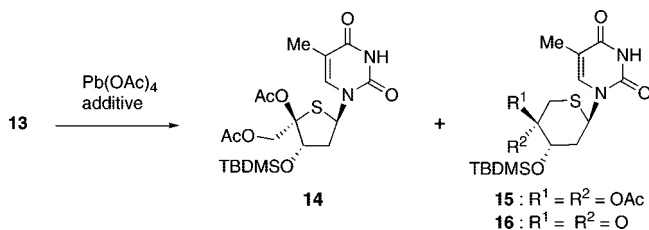
Scheme 4. Mechanism of Diacetoxylation of 13
