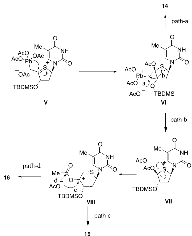
Scheme 4. Mechanism of Diacetoxylation of 13
