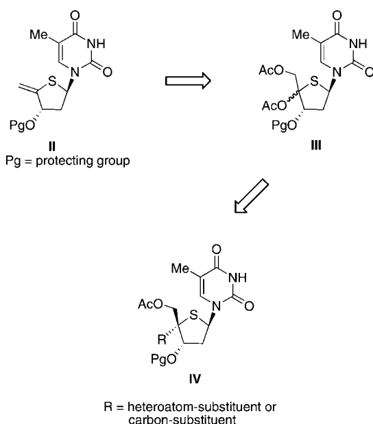
Scheme 2. Synthesis of 4',5'-Unsaturated 4'-Thiothymidines 12 and 13
