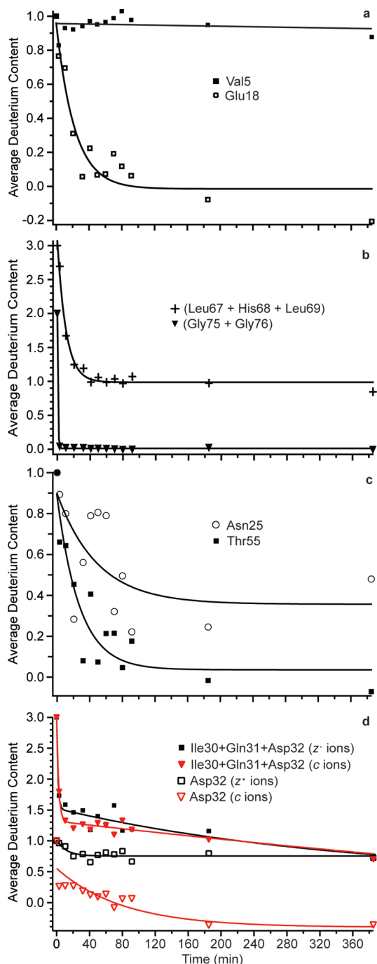
Figure 5. Example hydrogen/deuterium exchange kinetics, where single residue resolution was obtained for (a) Val5 and Glu18 and (b) a three-residue sum and a two-residue sum were obtained for Leu67, His68, and Leu69, and Gly75 and Gly76, respectively. Single residue resolution results for (c) Asn25 and Thr55 illustrate decay to different average deuterium content end points. Exchange kinetics for (d) Asp 32 plotted with c ion data (red) and z + ion data (black) and as part of a three-residue in silico digestion (Ile30 + Gln31 + Asp32). Data were fit to single or double exponential functions where appropriate.
