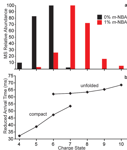
Figure 1. Plot of the (a) ESI-MS relative charge state abundances of 10 \mu M ubiquitin (20 mM aqueous ammonium acetate, pH 7.0) formed with and without 1% m -NBA and (b) TWIMS reduced arrival times as a function of charge state, which shows two distinct families of conformers.
