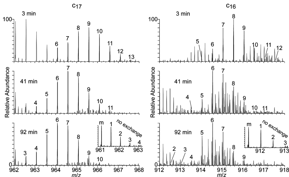
Figure 4. Partial ETD mass spectra of fully deuterated 10+ ubiquitin showing the c_{17} (left) and c_{16} (right) fragment ions obtained at 3, 41, and 92 min during exchange for hydrogen. The monoisotopic peak (m, inset) and each isotope peak in the distributions are labeled. Partial ETD spectra for the fully protonated c_{17} and c_{16} fragment ions obtained without HDX are in the inset.
